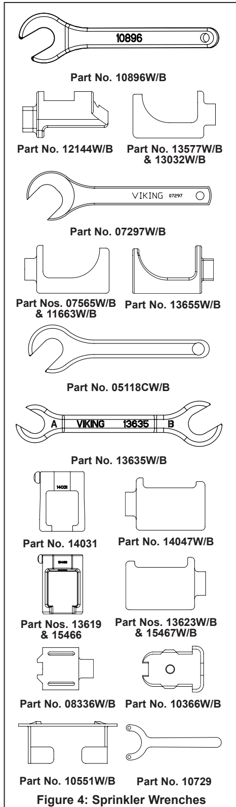
Figure 4: Sprinkler Wrenches
